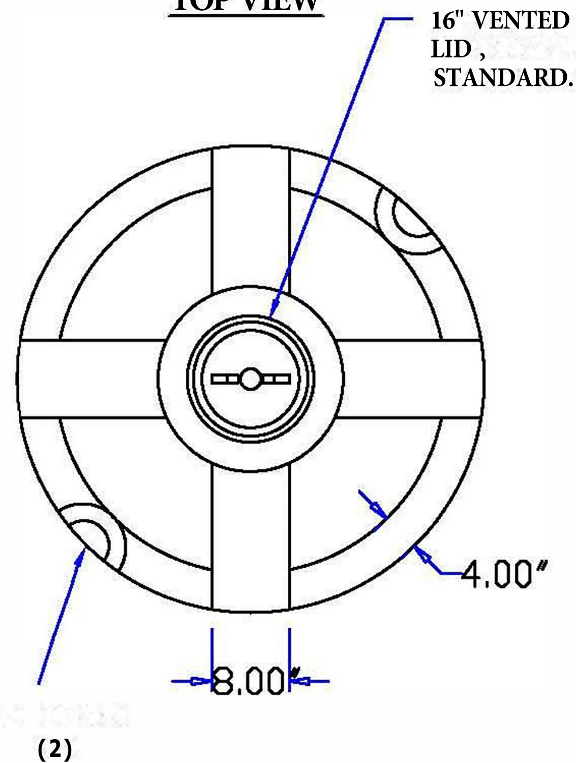
TOP VIEW
